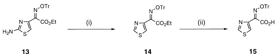
Scheme 3. Reagents: (i) tert -BuONO, THF, rt; (ii) NaOH, dioxane, H 2 O.
