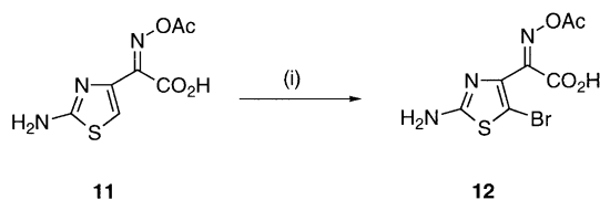
Scheme 2. Reagents and conditions; (i) NBS, MeOH, rt.
