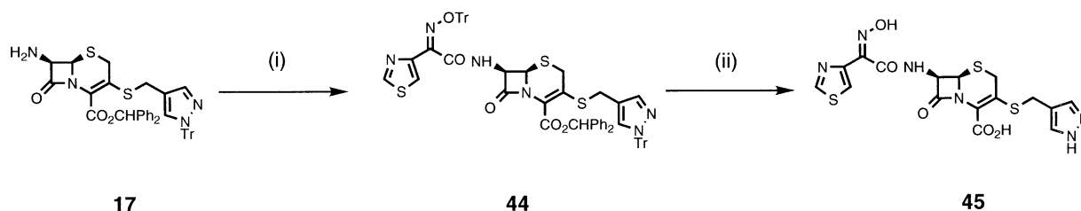
Scheme 5. Reagents: (i) (a) POCl 3 , DMF, AcOEt, THF; (b) 15 , BSA, CH 2 Cl 2 ; (ii) AlCl 3 , anisole, CH 3 NO 2 .
