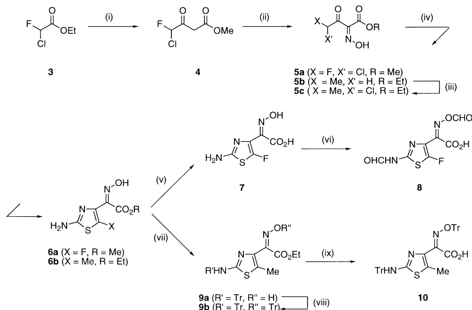
Scheme 1. Reagents and conditions: (i) (a) ClSO 3 H, phthaloyl chloride, 0 °C; (b) isopropylidene malonate, pyridine, 0 °C; (c) MeOH, reflux; (ii) isoamyl nitrate, CH 3 COCl, CH 2 Cl 2 , 0 °C–rt; (iii) SO 2 Cl 2 , AcOH, 0 °C–rt; (iv) thiourea, DMAc, 0 °C–rt; (v) BCl 3 , CH 2 Cl 2 , 0 °C; (vi) Ac 2 O, HCO 2 H, rt; (vii) TrCl, Et 3 N, DMF, rt; (viii) NaH, TrCl, AcOEt, rt; (ix) NaOH, dioxane, H 2 O, 100 °C.
